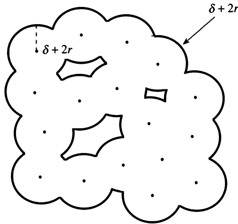
FIGURE 1: The outer curve is a contour \gamma = \gamma_{\omega, \omega'} of size 13. All the points pictured belong to \Psi(\omega') .
